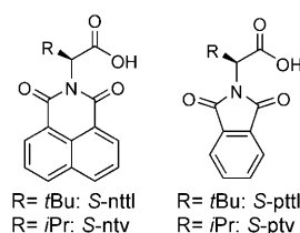
Figure 2. Ligands (L*H) for [\text{Rh}_2(\text{L}^*)_4] -catalyzed cyclopropanation. nttl = N -1,8-naphthoyl- tert -leucine; pttl = N -phthaloyl- tert -leucine; ntv = N -1,8-naphthoyl-valine; ptv = N -phthaloyl-valine.
